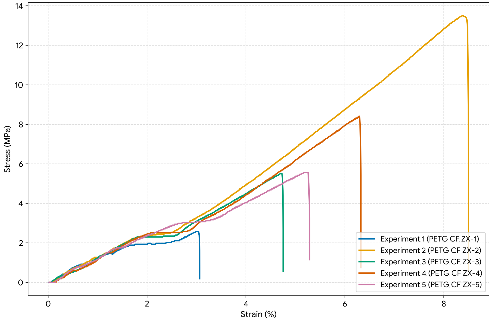
Stress-Strain Curves for PETG CF ZX (5 Experiments)
